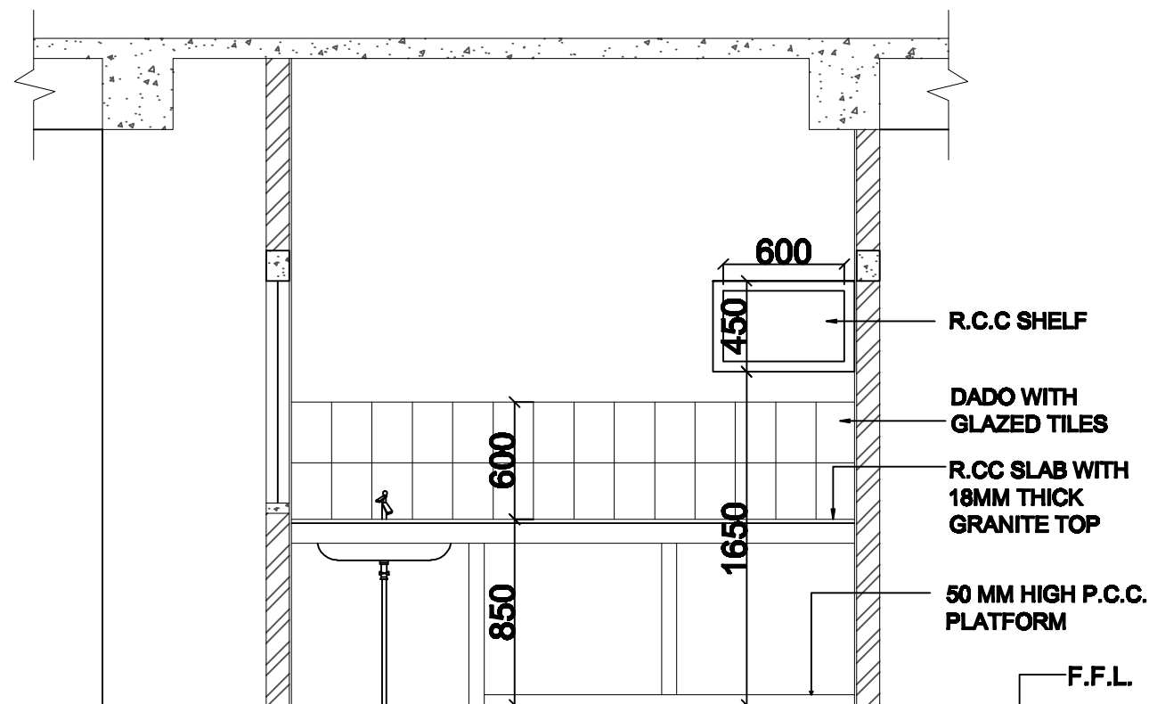
SECTION-YY
