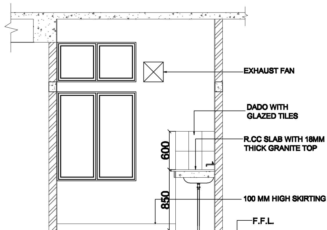
SECTION-XX
